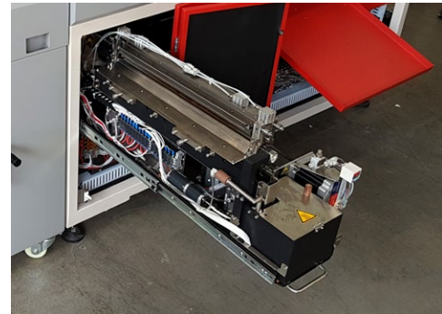
Hotmelt Walzenleimwerk
